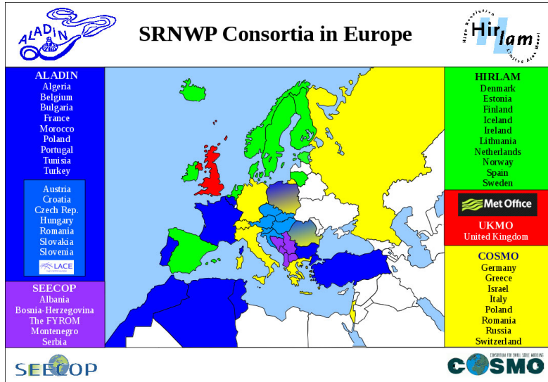
Figure 3: Short Range Numerical Weather Prediction (SRNWP) consortia in Europa, showing the participating countries in the HIRLAM (green) and ALADIN (blue) consortia (source: http://www.eumetnet.eu ).
