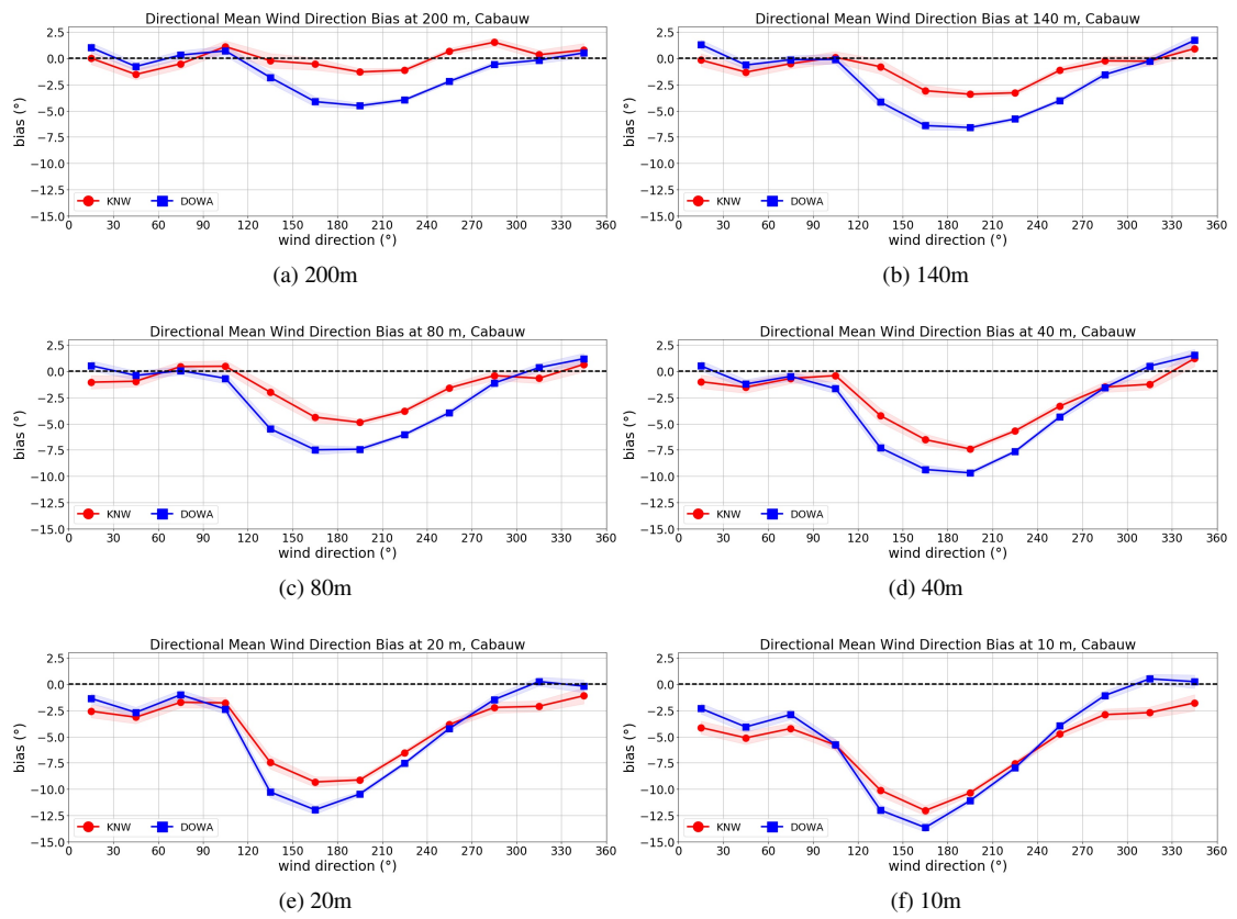
Figure 21: Directional wind direction bias, with sector width of 30^\circ , showing DOWA (blue) and KNW atlas (red). Note the different scales on the y-axis.
