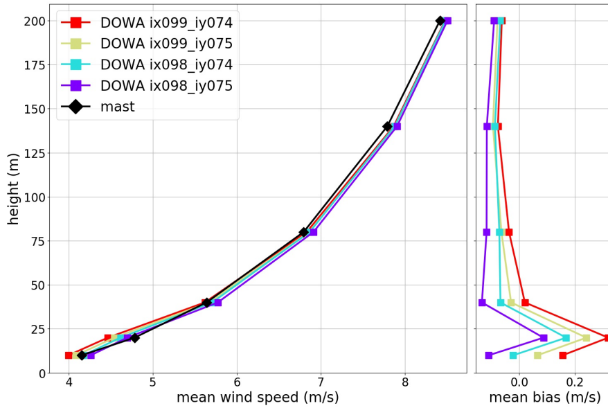
Figure 28: Height profile of the mean wind speed (left) and mean bias (right), showing mast measurements (black) and the four nearest grid points of DOWA.
