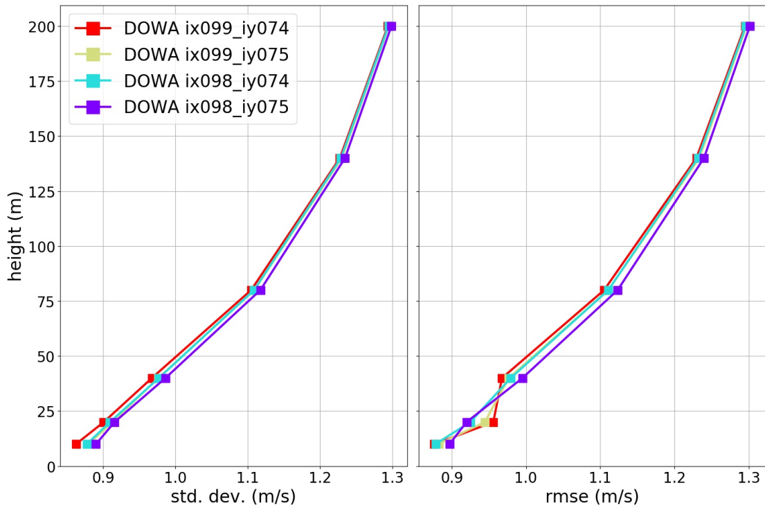
Figure 29: Height profile of the standard deviation of the bias (left) and root mean square error (rmse) (right), showing the four nearest grid points of DOWA.
