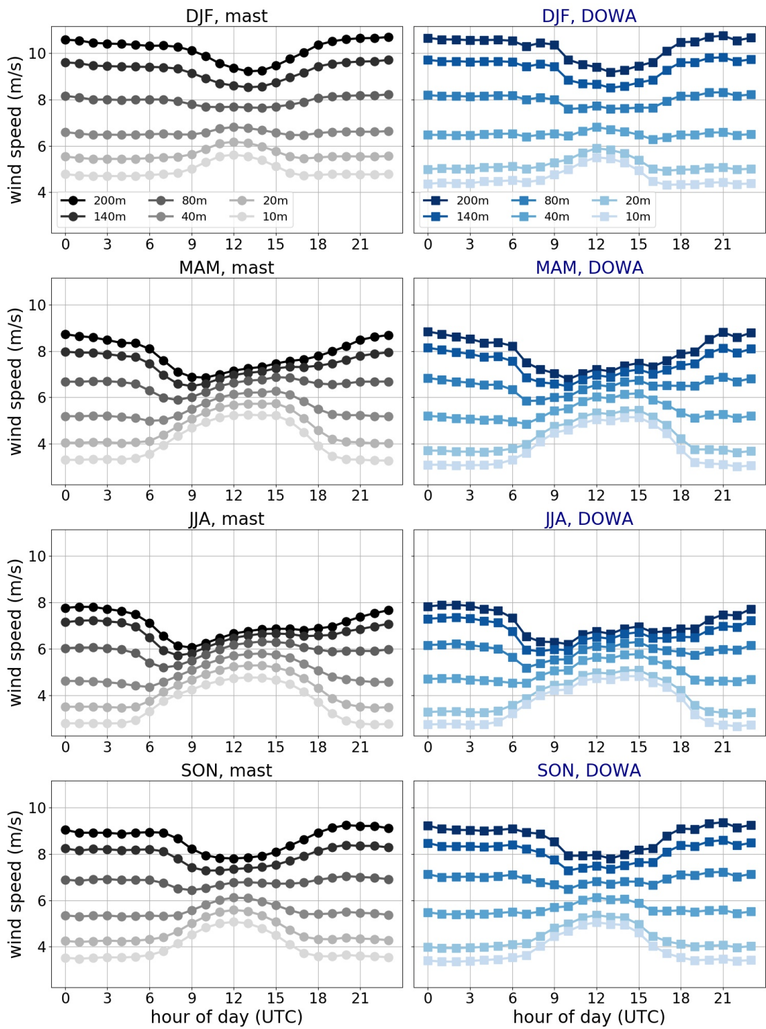
Figure 12: Hourly mean wind speed for the mast measurements (left) and DOWA (right), separated into the four season: winter (December, January, February), spring (March, April, May), summer (June, July, August) and autumn (September, October, November).
