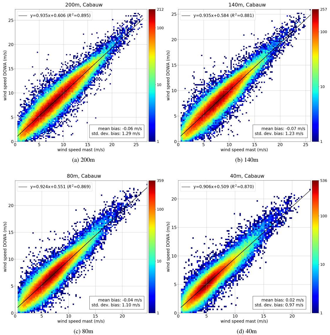
Figure 16: Scatterplot of the DOWA and mast wind speed data (visualized as a density plot with logarithmic color scale), showing the result of a linear regression (slope, intercept and R^2 ) and the mean bias and standard deviation of the bias.
