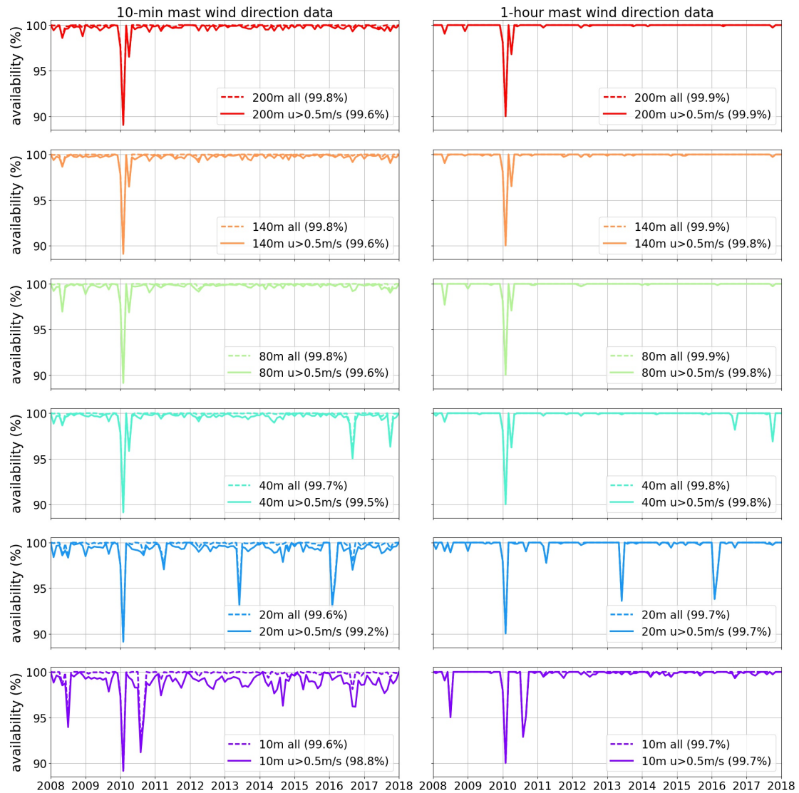
Figure 6: Monthly data availability of the 10-minute (left panel) and 1-hourly (right panel) wind direction measurements from the Cabauw meteor mast, all data (dashed lines) and data for which the wind speed is larger than 0.5 m/s (solid lines). In the legends the overall data availability per height for the whole period is given. Data availability is defined as the percentage of monthly valid 10-minute or hourly data, in which a valid hourly data requires only one valid 10-minute data.
