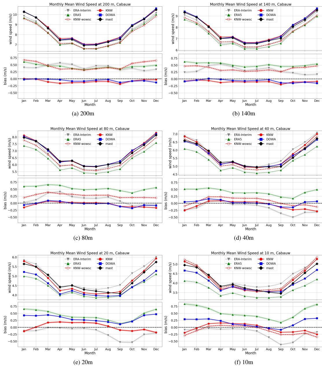
Figure 9: Monthly mean wind speed, showing mast measurements (black), DOWA (blue), KNW atlas (red), KNW atlas without wind shear correction (red, dashed), ERA5 (green, dotted) and ERA-Interim (gray, dotted). The upper panel shows the wind speed of both mast measurements and models, the lower panel the bias between the mast measurements and the models. Model variance is indicated by the shaded areas in the bias plots.
