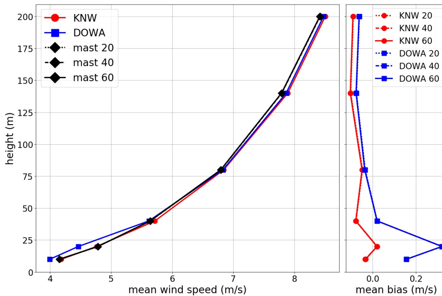
Figure 23: Height profile of the mean wind speed (left) and mean bias (right), showing mast measurements (black), DOWA (blue) and KNW atlas (red), for different averaging times (20, 40 and 60 minutes) of the mast measurements.
