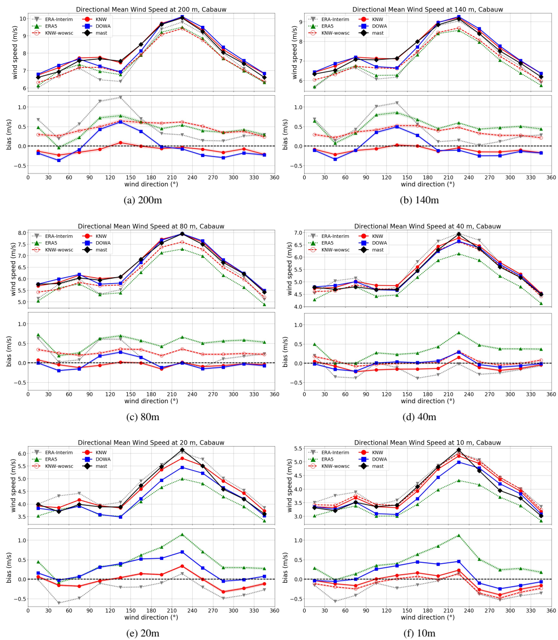
Figure 10: Directional mean wind speed, showing mast measurements (black), DOWA (blue), KNW atlas (red), KNW atlas without wind shear correction (red, dashed), ERA5 (green, dotted) and ERA-Interim (gray, dotted). The upper panel shows the wind speed of both mast measurements and models, the lower panel the bias between the mast measurements and the models. Model variance is indicated by the shaded areas in the bias plots.
