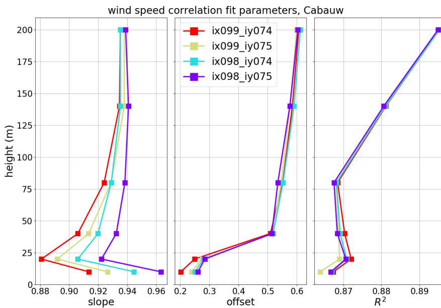
Figure 30: Height profile of the results of the linear regression (slope, offset and R^2 ) of the wind speed data, comparing the four nearest grid points of DOWA.
