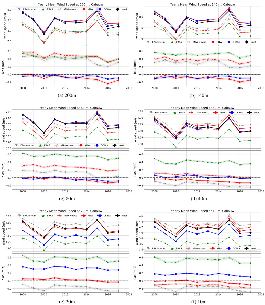
Figure 8: Yearly mean wind speed, showing mast measurements (black), DOWA (blue), KNW atlas (red), KNW atlas without wind shear correction (red, dashed), ERA5 (green, dotted) and ERA-Interim (gray, dotted). The upper panel shows the wind speed of both mast measurements and models, the lower panel the bias between the mast measurements and the models. Model variance is indicated by the shaded areas in the bias plots.
