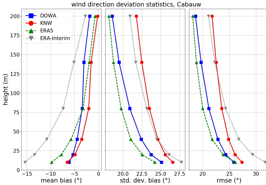
Figure 19: Height profile of the mean bias, standard deviation of the bias and rmse of the wind direction data: DOWA (blue), KNW atlas (red), ERA5 (green, dashed) and ERA-Interim (gray, dotted).
