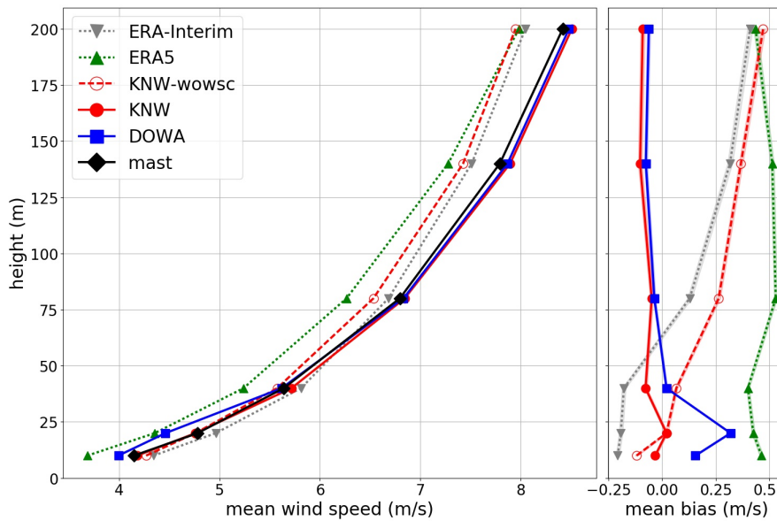
Figure 13: Height profile of the mean wind speed (left) and mean bias (right), showing mast measurements (black), DOWA (blue), KNW atlas (red), KNW atlas without windshear correction (red, dashed), ERA5 (green, dotted) and ERA-Interim (gray, dotted).
