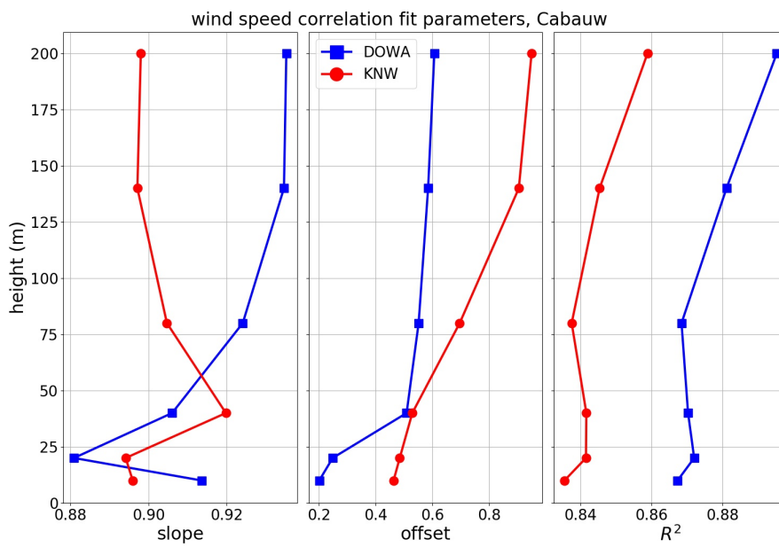
Figure 18: Height profile of the results of the linear regression (slope, offset and R^2 ) of the wind speed data, comparing the DOWA (blue) and KNW atlas (red).
