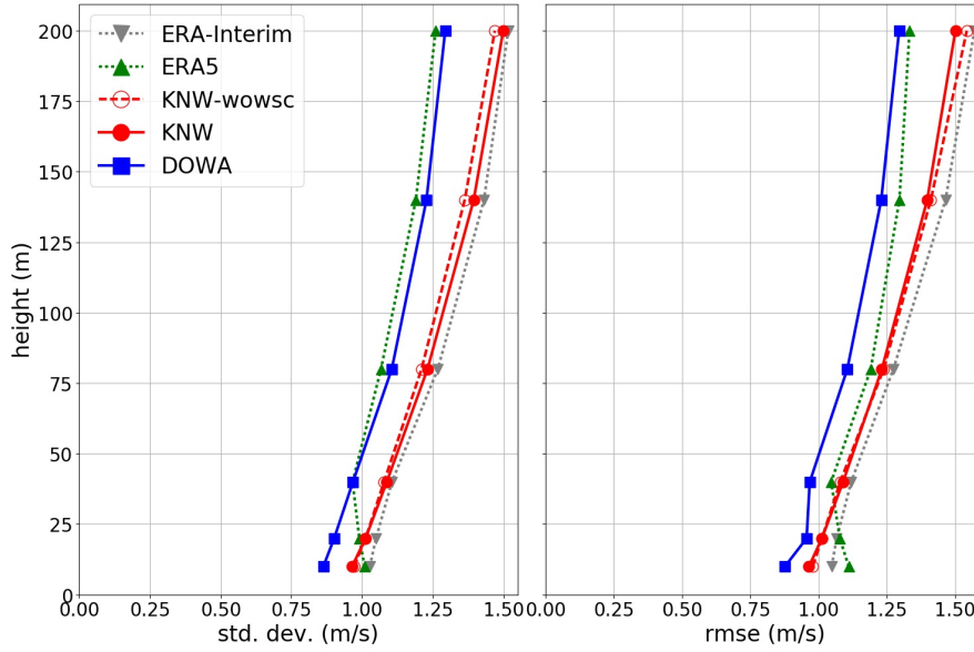
Figure 14: Height profile of the standard deviation of the bias (left) and root mean square error (rmse) (right), showing DOWA (blue), KNW (red), KNW without windshear correction (red, dashed), ERA5 (green, dotted) and ERA-Interim (gray, dotted).
