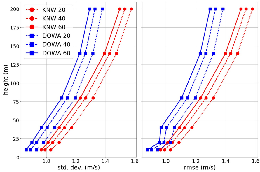
Figure 24: Height profile of the standard deviation of the bias (left) and root mean square error (rmse) (right), showing DOWA (blue) and KNW (red), for different averaging times (20, 40 and 60 minutes) of the mast measurements.
