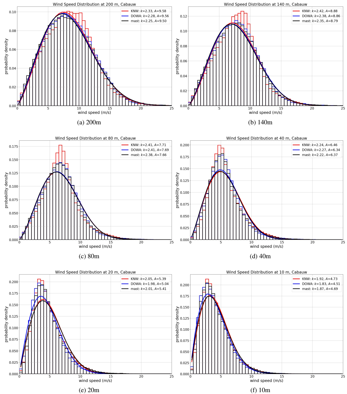
Figure 33: Wind speed distributions, with bin width of 0.5 m/s, showing mast measurements (black), DOWA (blue) and KNW (red) and corresponding Weibull fits (resulting fit parameters indicated in the legends).
