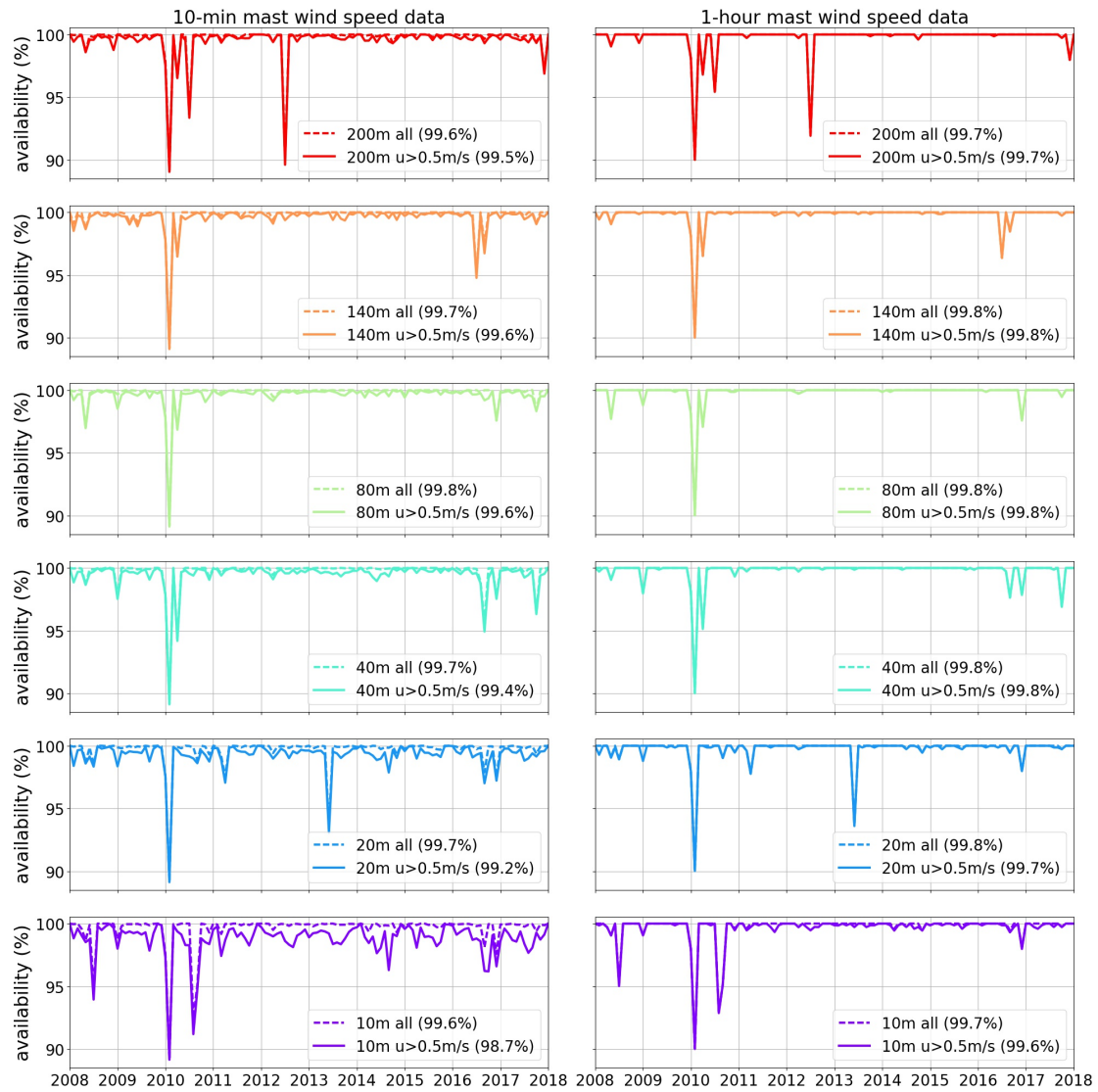
Figure 5: Monthly data availability of the 10-minute (left panel) and 1-hourly (right panel) wind speed measurements from the Cabauw meteor mast, all data (dashed lines) and data for which the wind speed is larger than 0.5 m/s (solid lines). In the legends the overall data availability per height for the whole period is given. Data availability is defined as the percentage of monthly valid 10-minute or hourly data, in which a valid hourly data requires only one valid 10-minute data.
