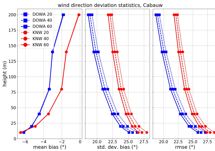
Figure 26: Height profile of the mean bias, standard deviation of the bias and rmse of the wind direction data, comparing the DOWA (blue) and KNW atlas (red), for different averaging times (20, 40 and 60 minutes) of the mast measurements.
