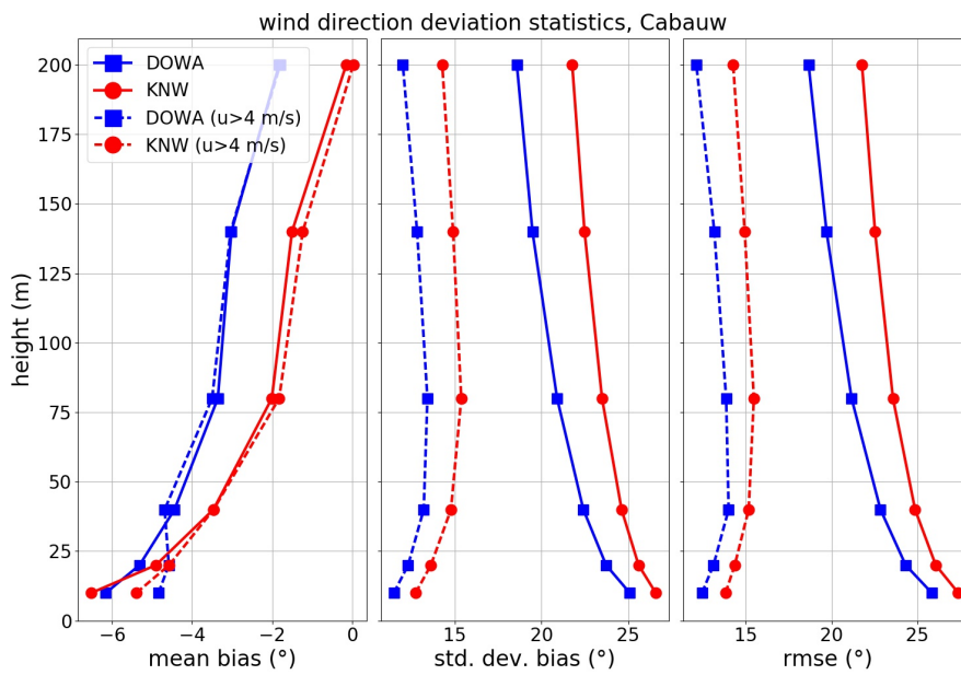
Figure 20: Height profile of the mean bias, standard deviation of the bias and rmse of the wind direction data, comparing the DOWA (blue) and KNW atlas (red). Solid lines are all data, dashed lines only data with wind speed larger than 4 m/s.
