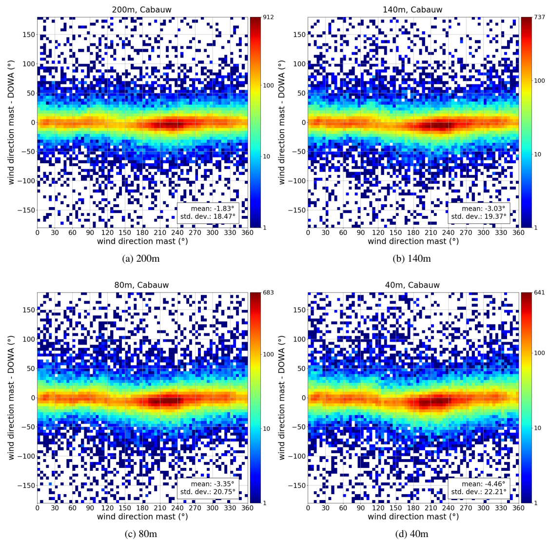
Figure 34: Scatterplot of the DOWA and mast wind direction data (visualized as a density plot with logarithmic color scale), showing the mean and standard deviation of the difference between the mast measurements and DOWA.
