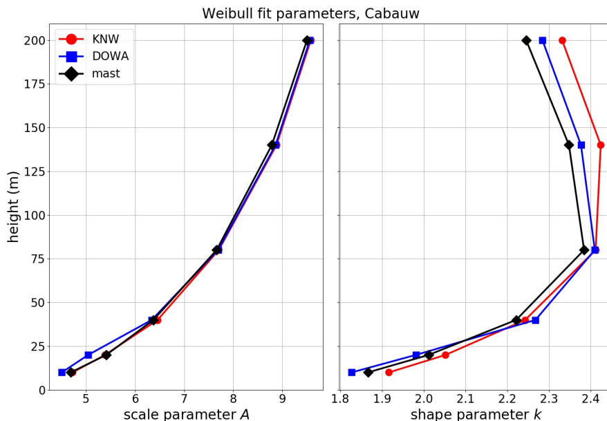
Figure 15: Height profiles of the Weibull scale parameter A (left) and shape parameter k (right), showing mast measurements (black), DOWA (blue) and KNW atlas (red).
