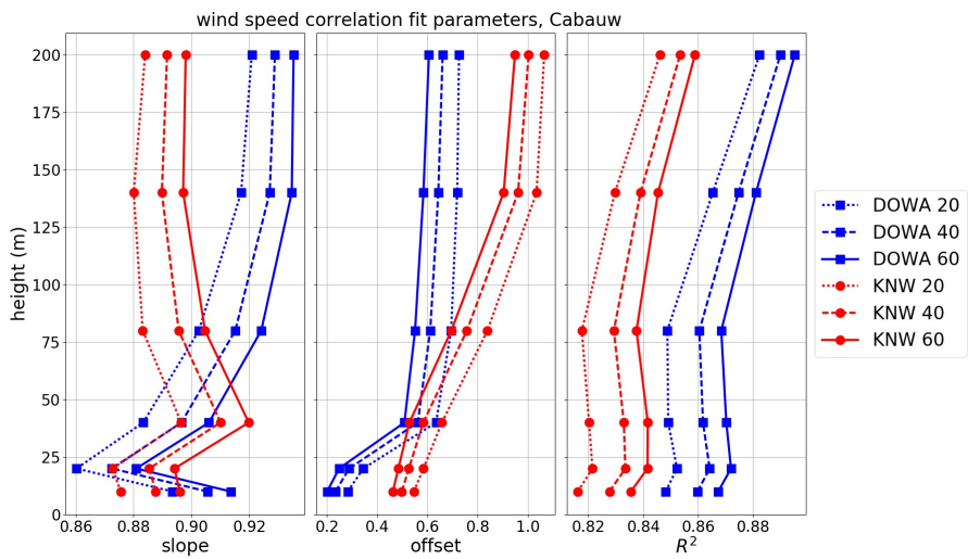
Figure 25: Height profile of the results of the linear regression (slope, offset and R^2 ) of the wind speed data, comparing the DOWA (blue) and KNW atlas (red), for different averaging times (20, 40 and 60 minutes) of the mast measurements.
