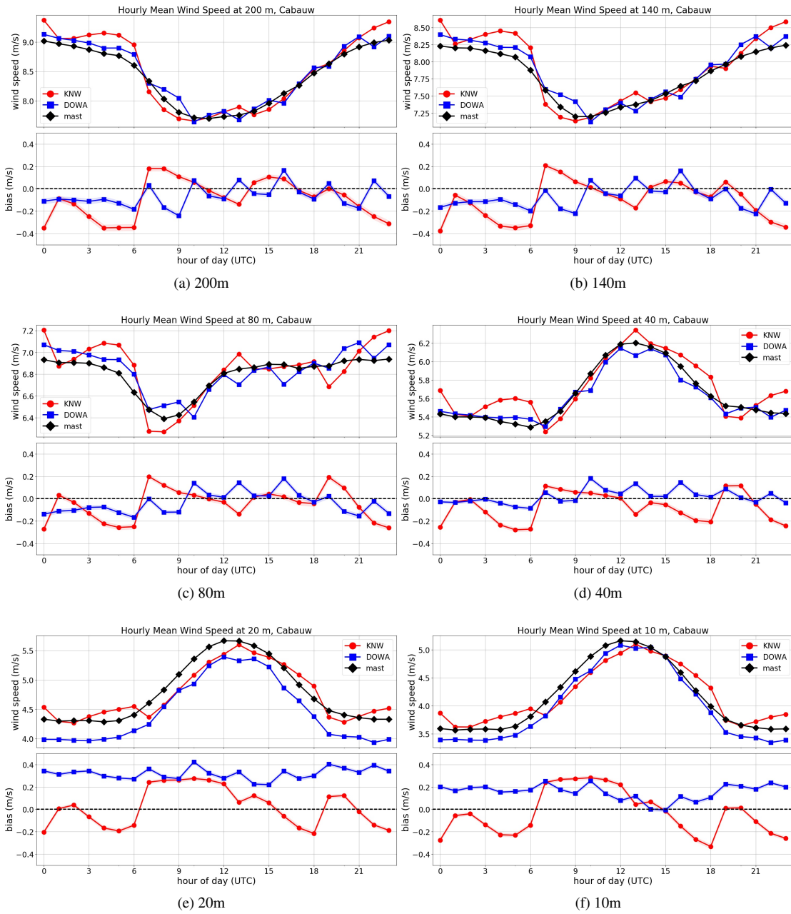
Figure 11: Hourly mean wind speed, showing mast measurements (black), DOWA (blue) and KNW atlas (red). The upper panel shows the wind speed of both mast measurements and models, the lower panel the bias between the mast measurements and the models.
