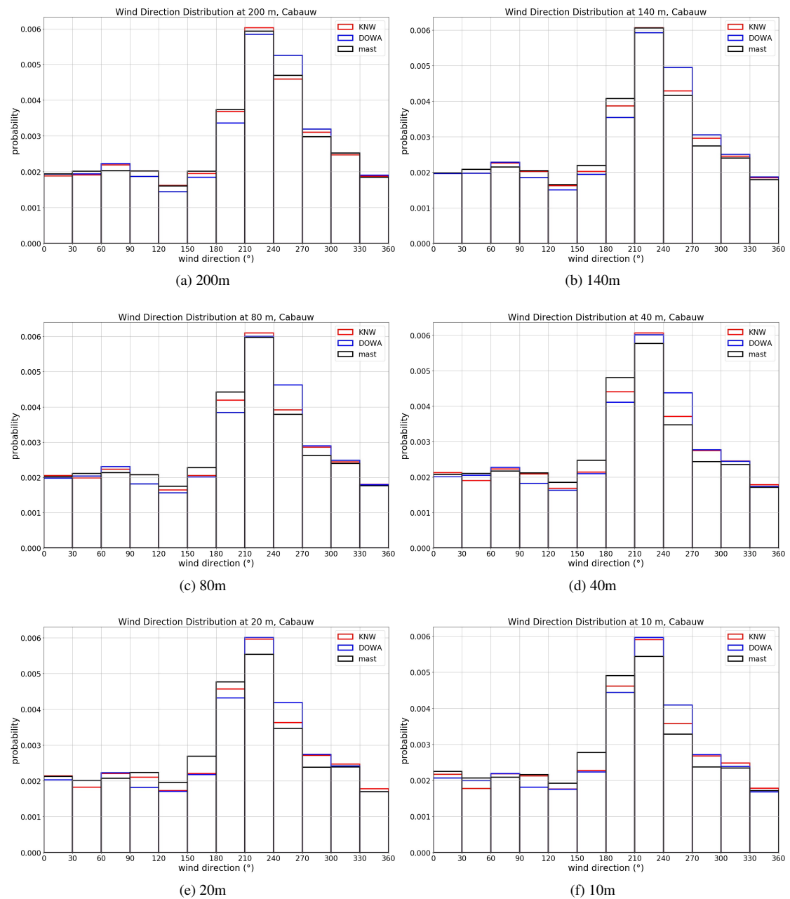
Figure 32: Wind direction distributions, with sector width of 30^\circ , showing mast measurements (black), DOWA (blue) and KNW (red).
