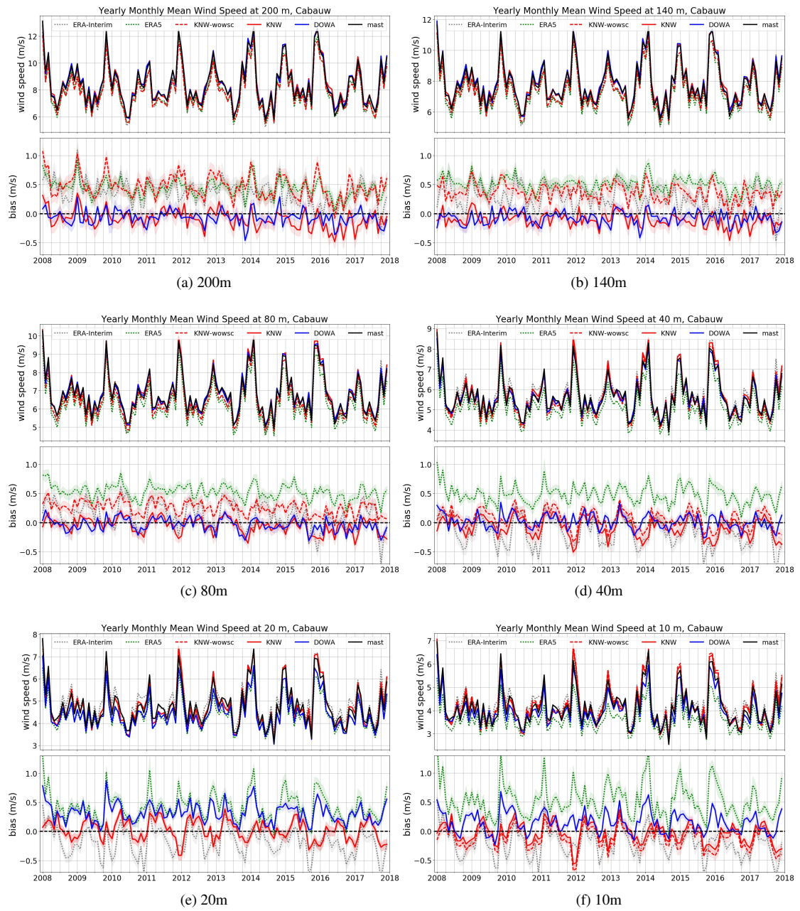
Figure 7: Yearly monthly mean wind speed, showing mast measurements (black), DOWA (blue), KNW atlas (red), KNW atlas without wind shear correction (red, dashed), ERA5 (green, dotted) and ERA-Interim (gray, dotted). Model variance is indicated by the shaded areas in the bias plots.
