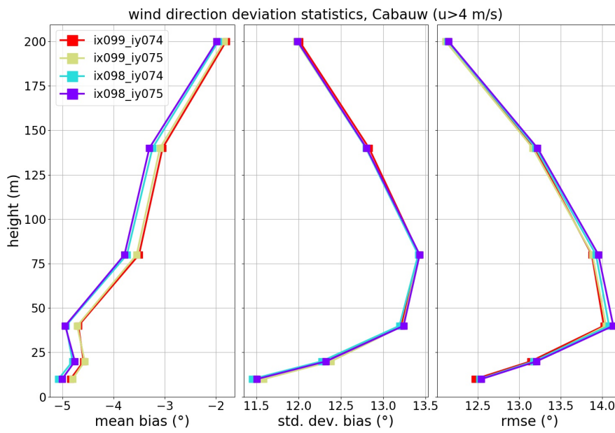
Figure 31: Height profile of the mean bias, standard deviation of the bias and rmse of the wind direction data, comparing the four nearest grid points of DOWA.
