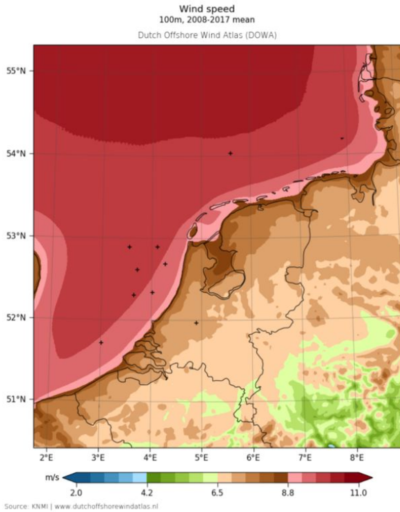
Figure 1: Sample picture from the DOWA website [1], showing the 10-year (2008-2017) average wind speed at a height of 100 m. The only symbol inland indicates the location of Cabauw (51.97°N, 4.93°E).
