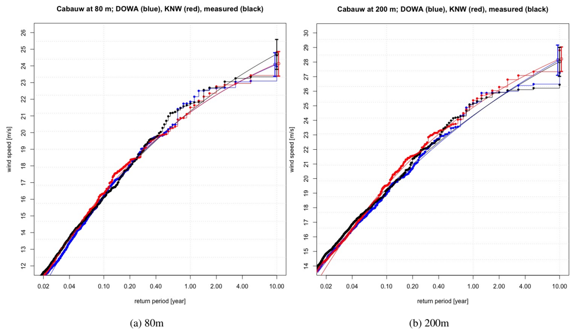
Figure 22: Extreme value analysis, showing the wind speed as function of return period for the mast measurements (black dots), DOWA (blue dots) and KNW atlas (red dots) for (a) 80 m and (b) 200 m. The solid lines (without the dots) are the results of a GPD (General Parato Distribution) fit to the data. For the last data points at 10 year return period the uncertainty (90% confidence level) is indicated by the vertical error bars.
